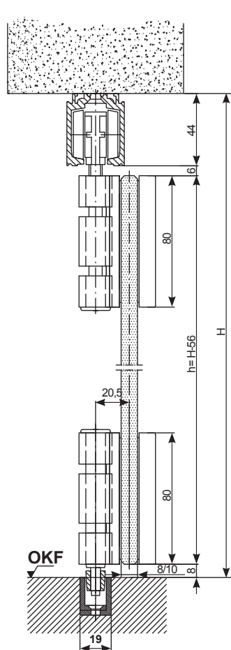
Vertical section
