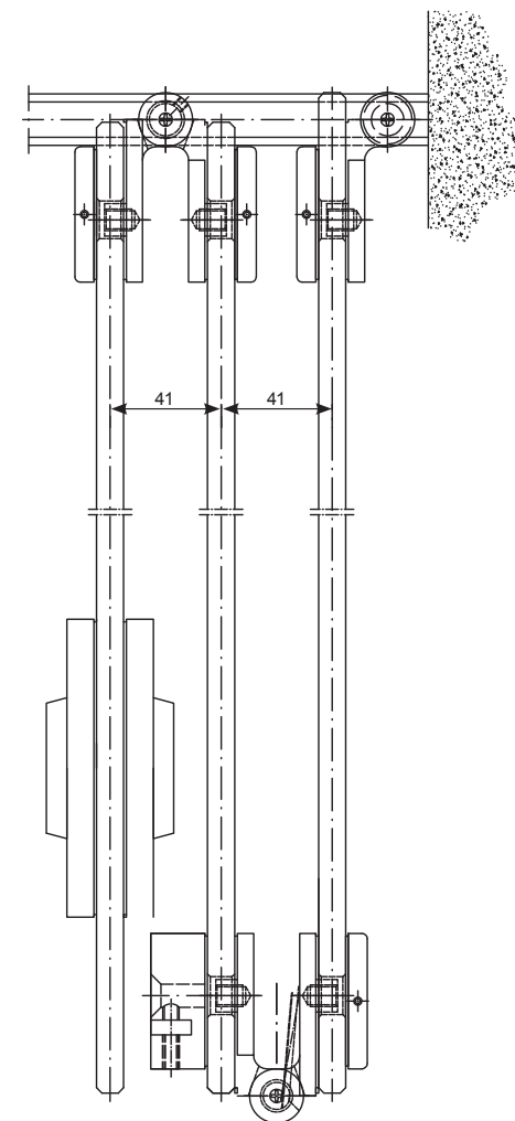
Horizontal section
